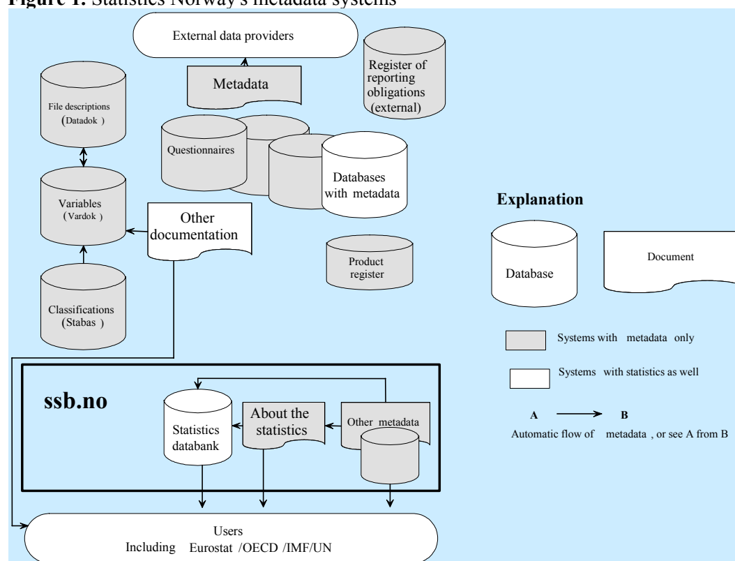
Figure 1. Statistics Norway's metadata systems
