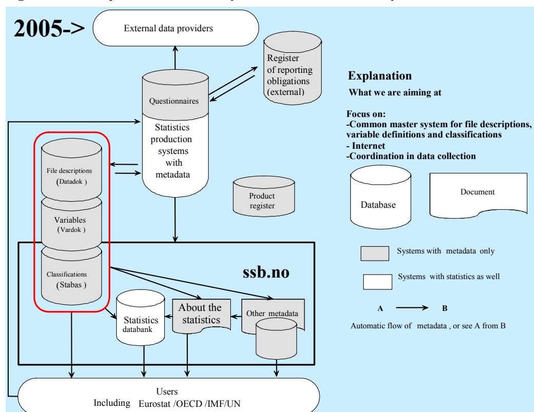
Figure 2. Development of metadata systems in Statistics Norway
